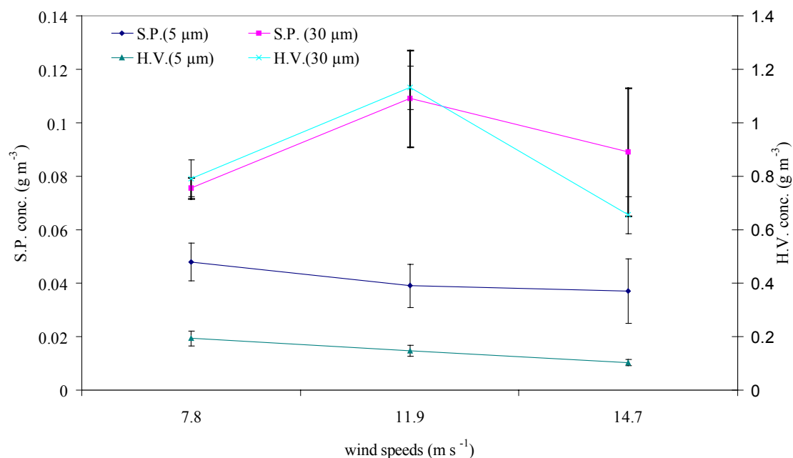
Figure 3. Concentrations of 5 and 30 \mu\text{m} materials measured by a shrouded probe (S.P.) and high volume sampler (H.V.) in a wind tunnel
