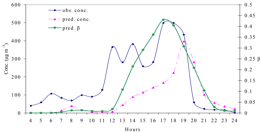
Figure 4. Temporal variations of \beta , observed and predicted PM_{10} concentrations at Crown Zellerbach (CZ), September 11, 1993
