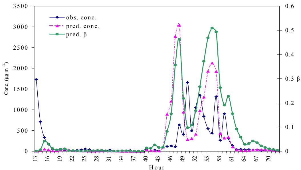
Figure 3. Temporal variations of \beta , observed and predicted PM_{10} concentrations at Kennewick (KW), September 23 to 25, 1999
